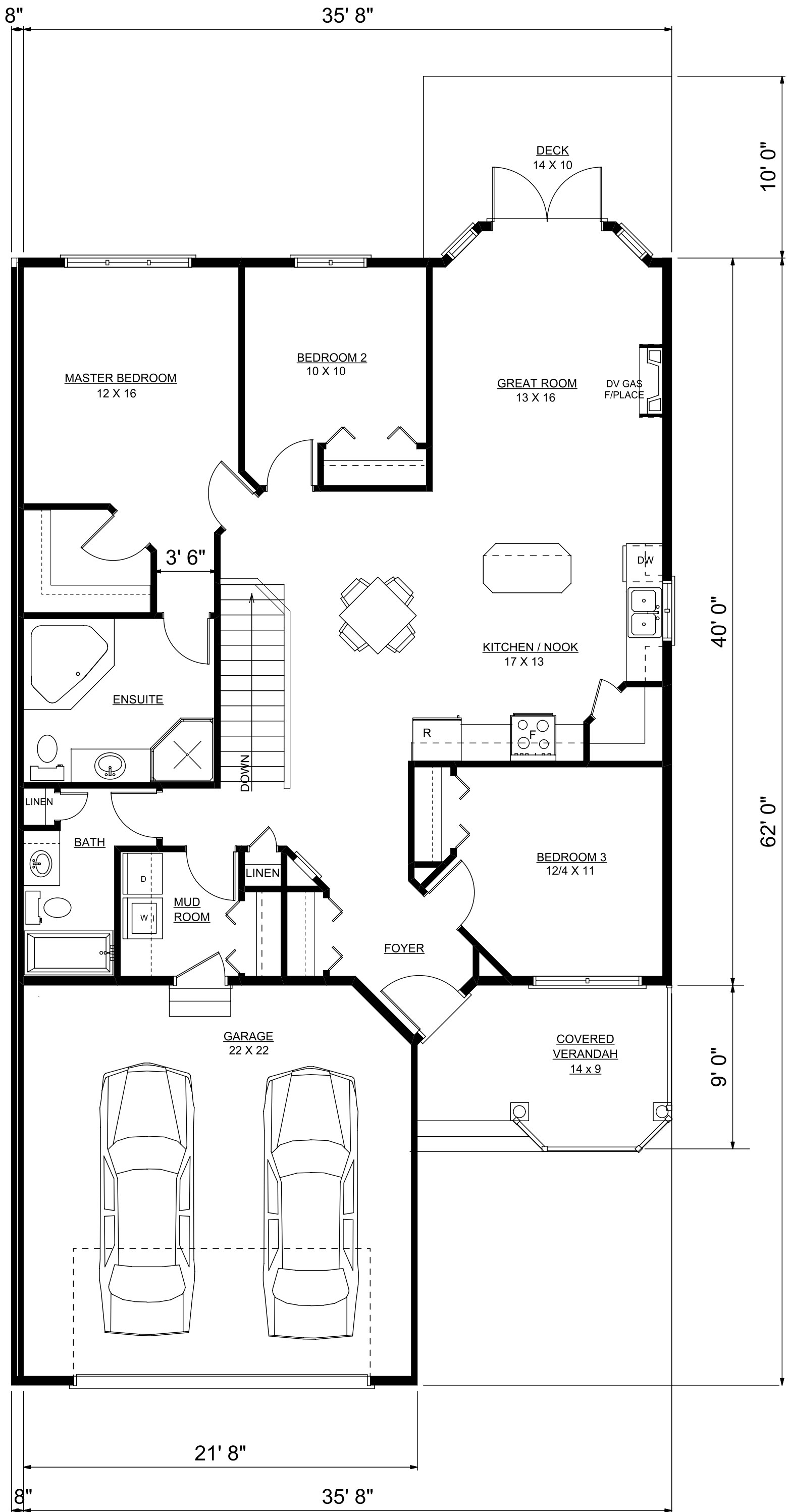
THREE BEDROOM BUNGALOW AREA = 1470 S.F.
