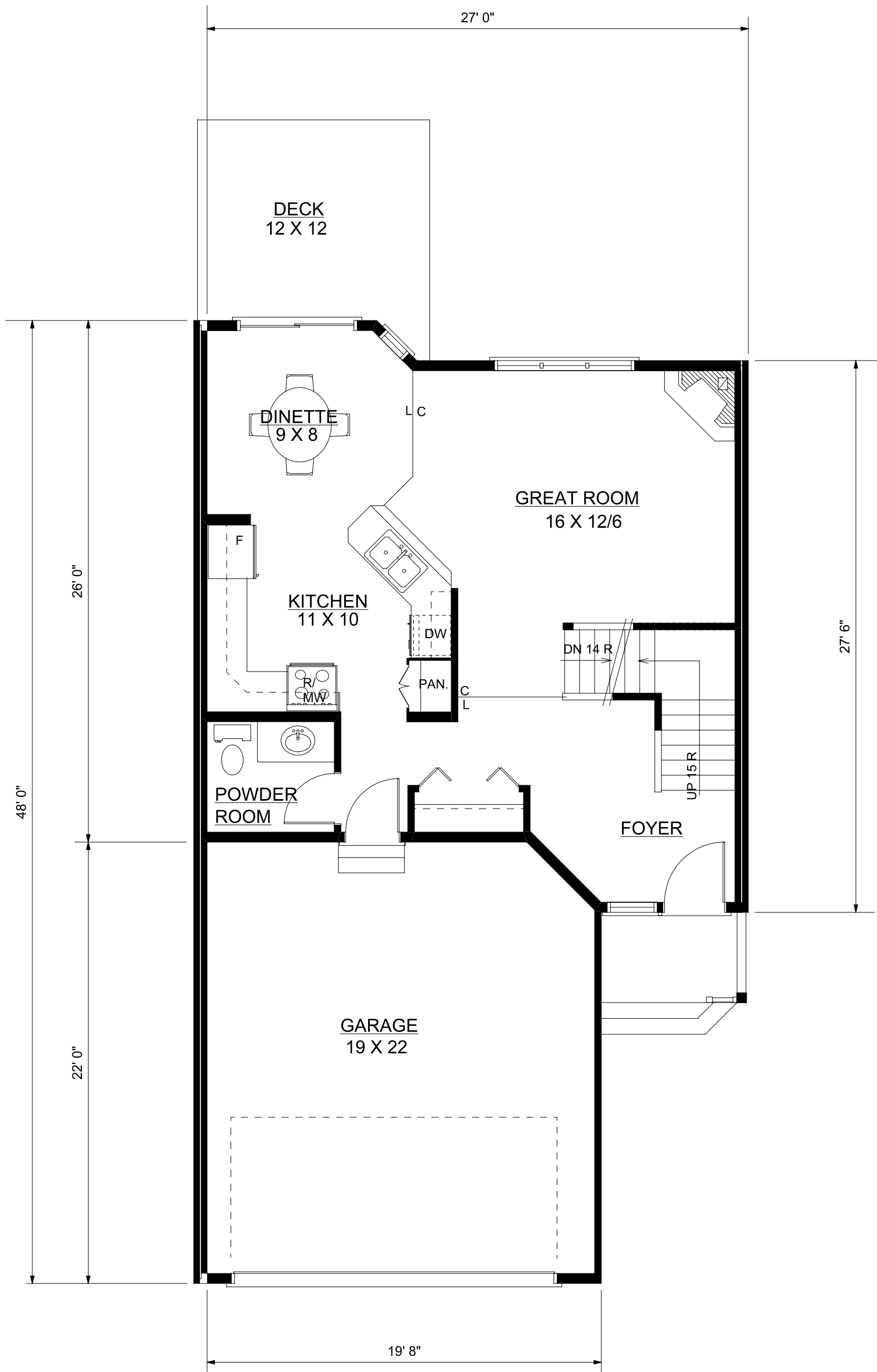
MAIN FLOOR PLAN 700 SQ. FT.
